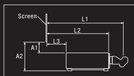
PT-RW630 with ET-DLE030 (16:10 aspect ratio) unit: meters (feet)
