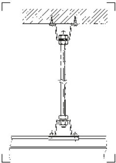
RAIL MOUNTING KIT WITH M12 STUD FF3214B
