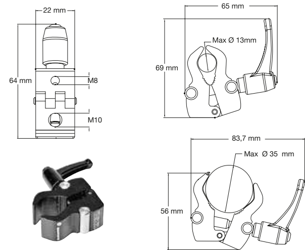
NANO CLAMP 386B-1
