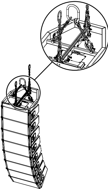
V8/V12 array with Z5380 V Flying frame 2 x Z5381 V Hoist connector chain Z5382 V Safety chainset
