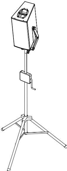
V7P/V10P with Z5383 VP Mounting bracket Z5024 Loudspeaker stand adapter Z5009 Loudspeaker stand with winder
