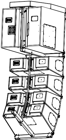
Vi array with Z5380 V Flying frame Z5387.001 Vi Mounting frame bottom (2pcs)
