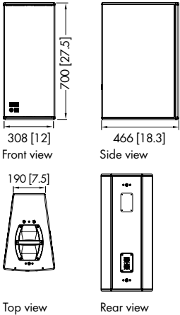
V10P cabinet dimensions in mm [inch]
