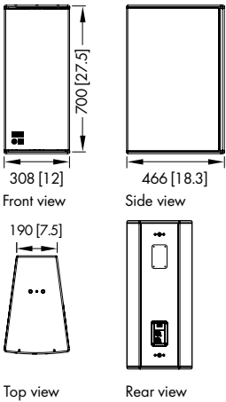
Vi10P cabinet dimensions in mm [inch]
