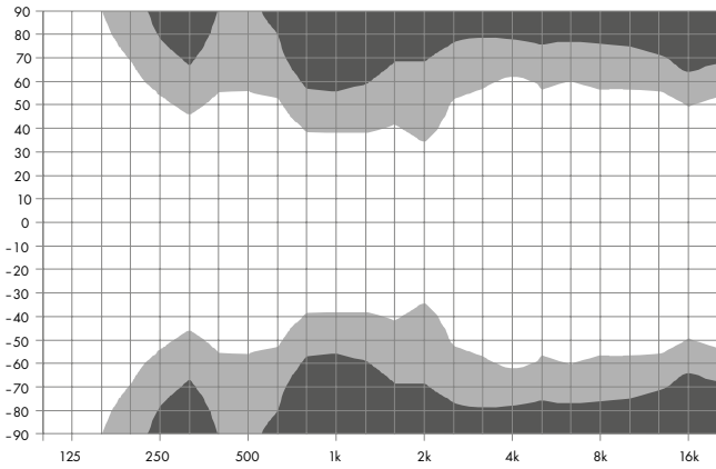
V12 and Vi12 horizontal dispersion characteristics 2
