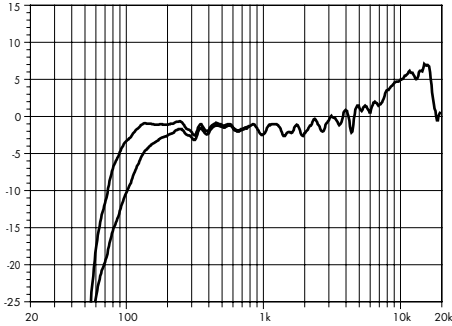
V12/Vi12 standard and CUT (single cabinet)
