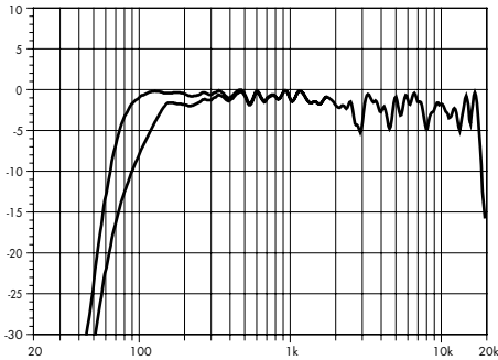
V10/Vi10P standard and CUT (single cabinet)
