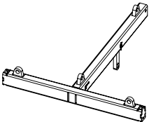
Z5387.000 Vi Mounting frame top For a maximum load equivalent to four Vi8/Vi12 loudspeakers 141 kg (311 lb)
