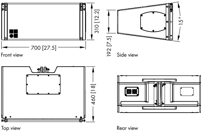
Vi12 cabinet dimensions in mm [inch]
