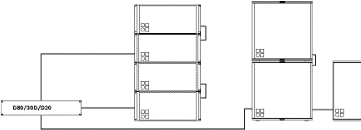
D80/30D/D20 amplifier in a mixed configuration of Dual Channel and Mix TOP/SUB mode for V7P, V10P, Vi7P, Vi10P, V8, V12, Vi8, Vi12 as well as V-GSUB, Vi-GSUB, V-SUB and Vi-SUB
