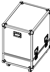
E7465 Touring case 2 x V Flying frame Dimensions (H x W x D): 970 x 800 x 600 mm 38.2 x 31.5 x 23.6 inch Net weight: 52 kg (120 lb)
