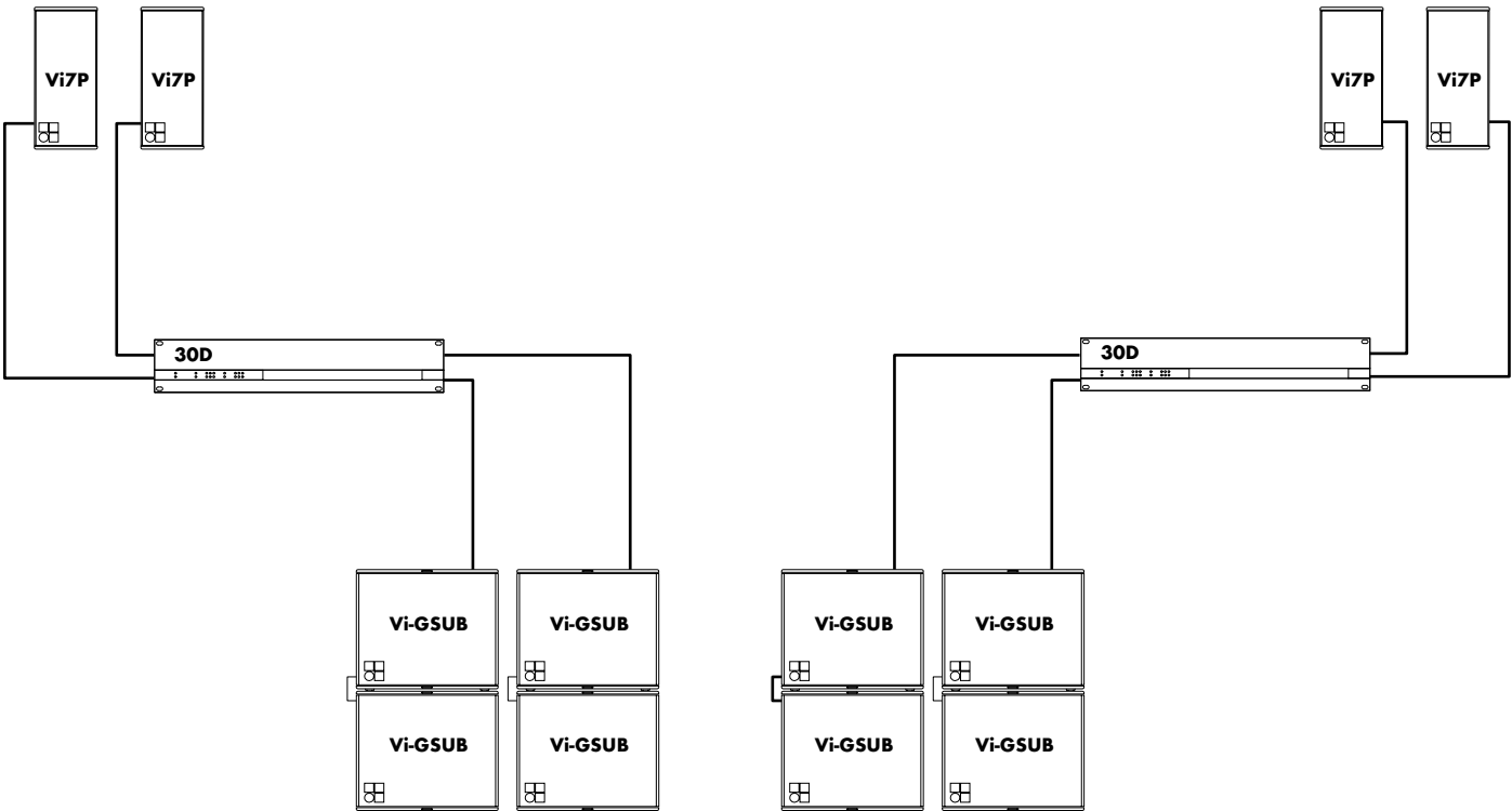
Vi7P loudspeakers in a distributed point source system and ground stacked Vi-GSUBs, with 30D amplifiers in Dual Channel mode
