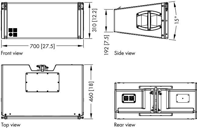
V12 cabinet dimensions in mm [inch]
