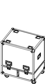
E7462 Touring case 2 x V8/V12 Dimensions (H x W x D): 900 x 800 x 600 mm 35.4 x 31.5 x 23.6 inch Net weight: 40 kg (88 lb)
