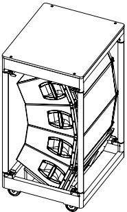
E7463 Touring cart 4 x V8/V12 Dimensions (H x W x D): 1420 x 700 x 800 mm 56 x 27.5 x 31.5 inch Total weight: 190 kg (420 lb) Maximum top load: 100 kg (220 lb)
