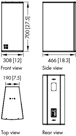
Vi7P cabinet dimensions in mm [inch]
