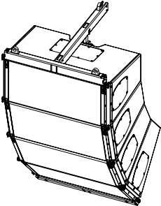
Vi8/Vi12 array with Z5387.001 Vi Mounting frame top Z5387.000 Vi Mounting frame bottom
