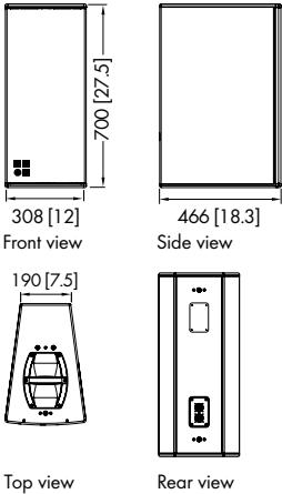
V7P cabinet dimensions in mm [inch]
